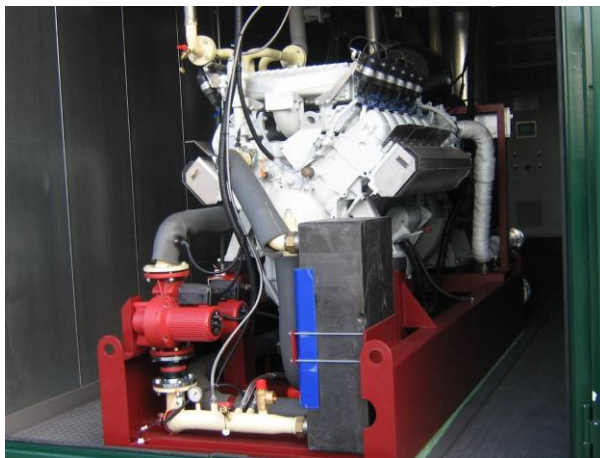
Inside CHP, a gas motor
